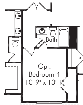
Optional Main Level At Optional Fourth Bedroom
